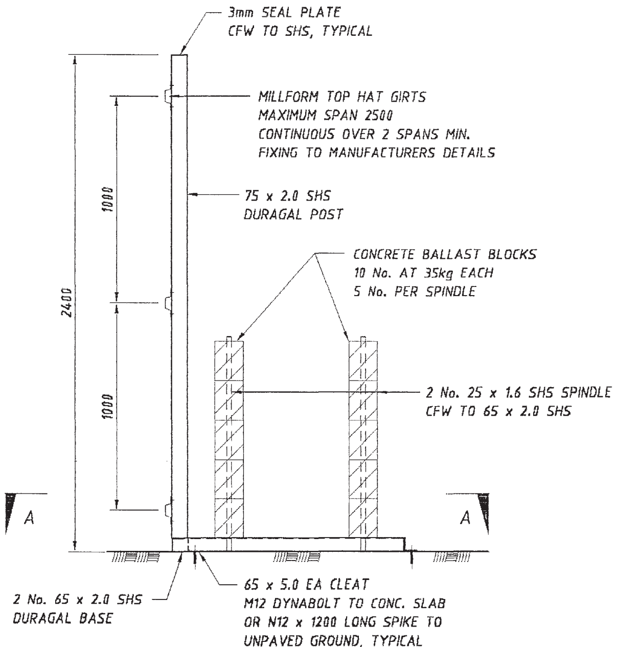
SIDE VIEW
